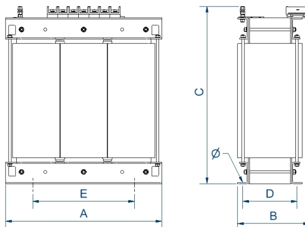
Dimensiones (AxBxCxDxE): 640x370x500x199,5x426 mm 11Ø
