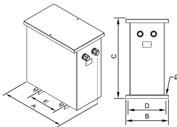
Dimensions (AxBxCxDxE): 724x410x764x370x350 mm 11Ø
