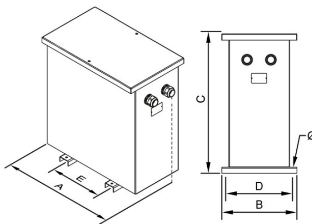
Dimensions (AxBxCxDxE): 970x621x1142x500x426 mm 12Ø
