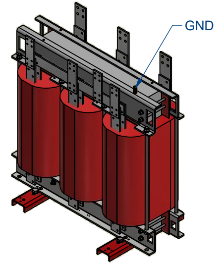
AUTW1000 Transformer ( 1/25 )
