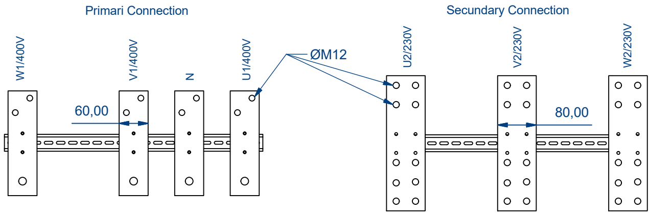
AUTW630 Transformer ( 1/20 )
