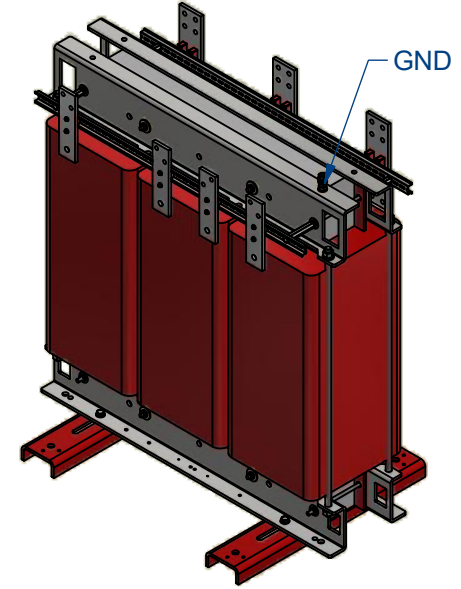
AUTW630 Transformer ( 1/20 )
