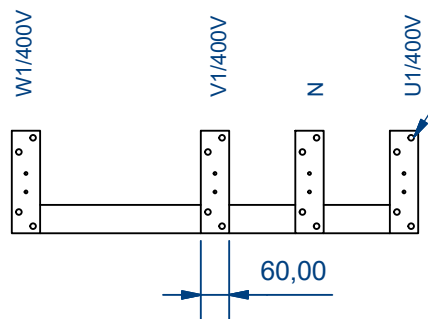
AUTW800 Enclosure ( 1/30 )
