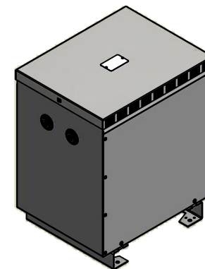
TKW25 Enclosure ( 1/18 )
